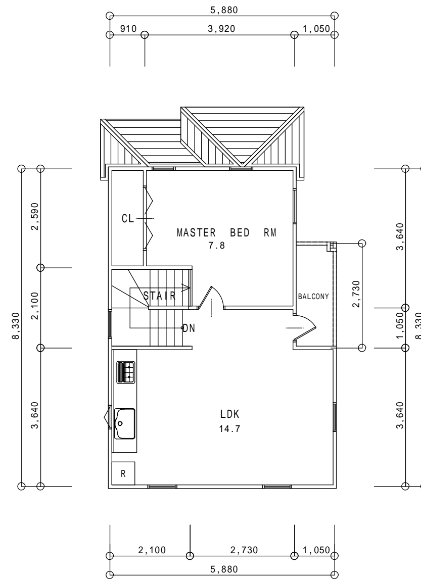
2nd FLOOR PLAN S:1/100
