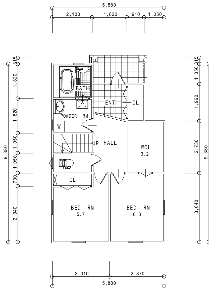
1st FLOOR PLAN S:1/100
