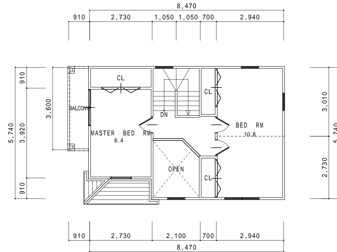
2nd FLOOR PLAN S:1/100
