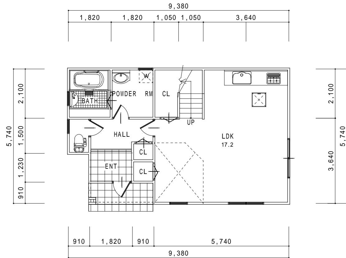
1st FLOOR PLAN S:1/100
