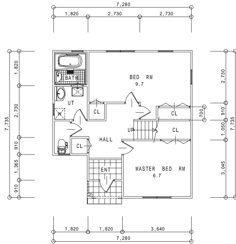
1st FLOOR PLAN S:1/100
