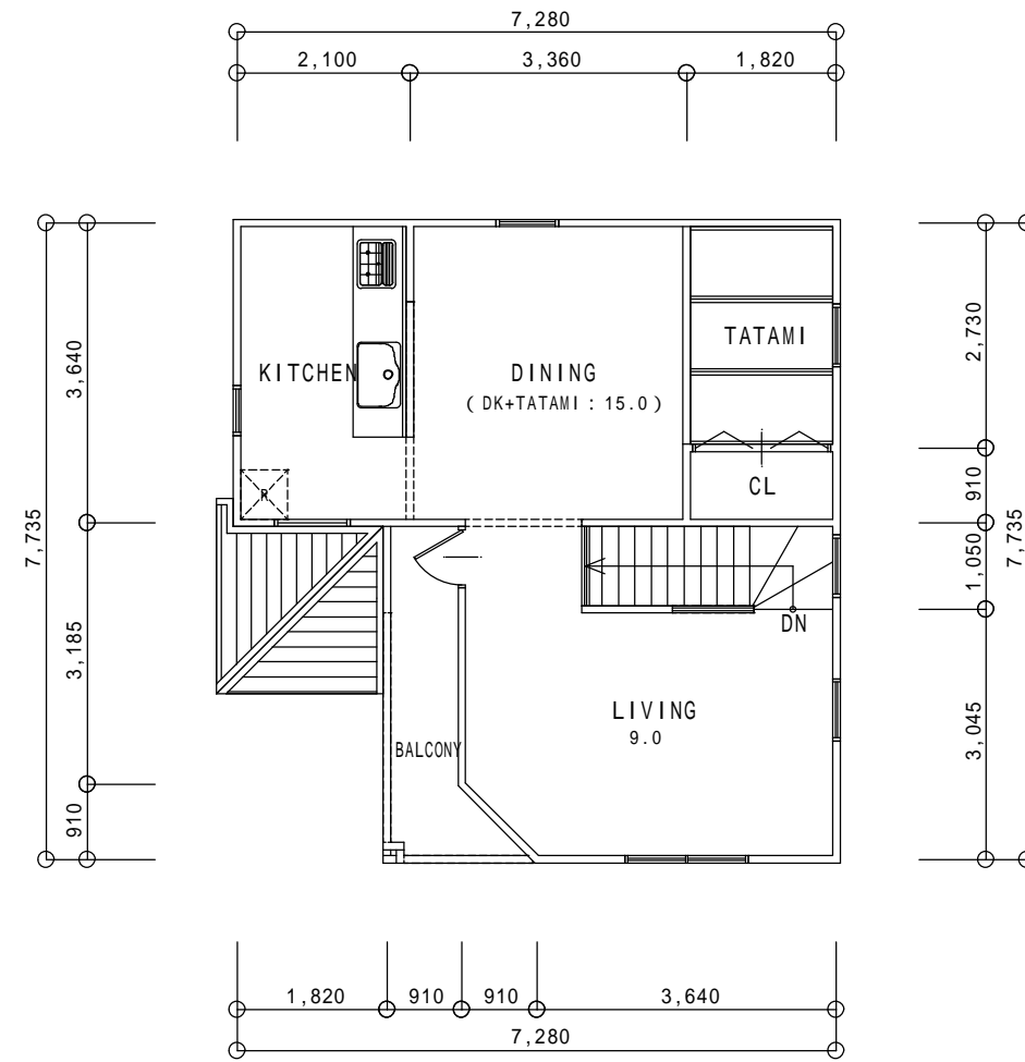
2nd FLOOR PLAN S:1/100
