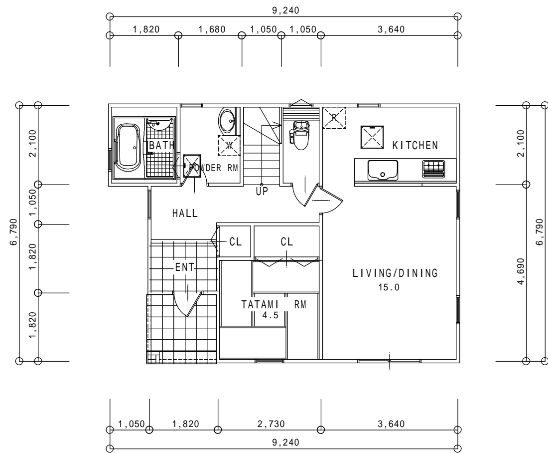
1st FLOOR PLAN S : 1/ 100
