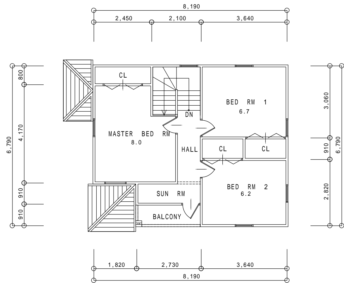
2nd FLOOR PLAN S : 1/ 100
