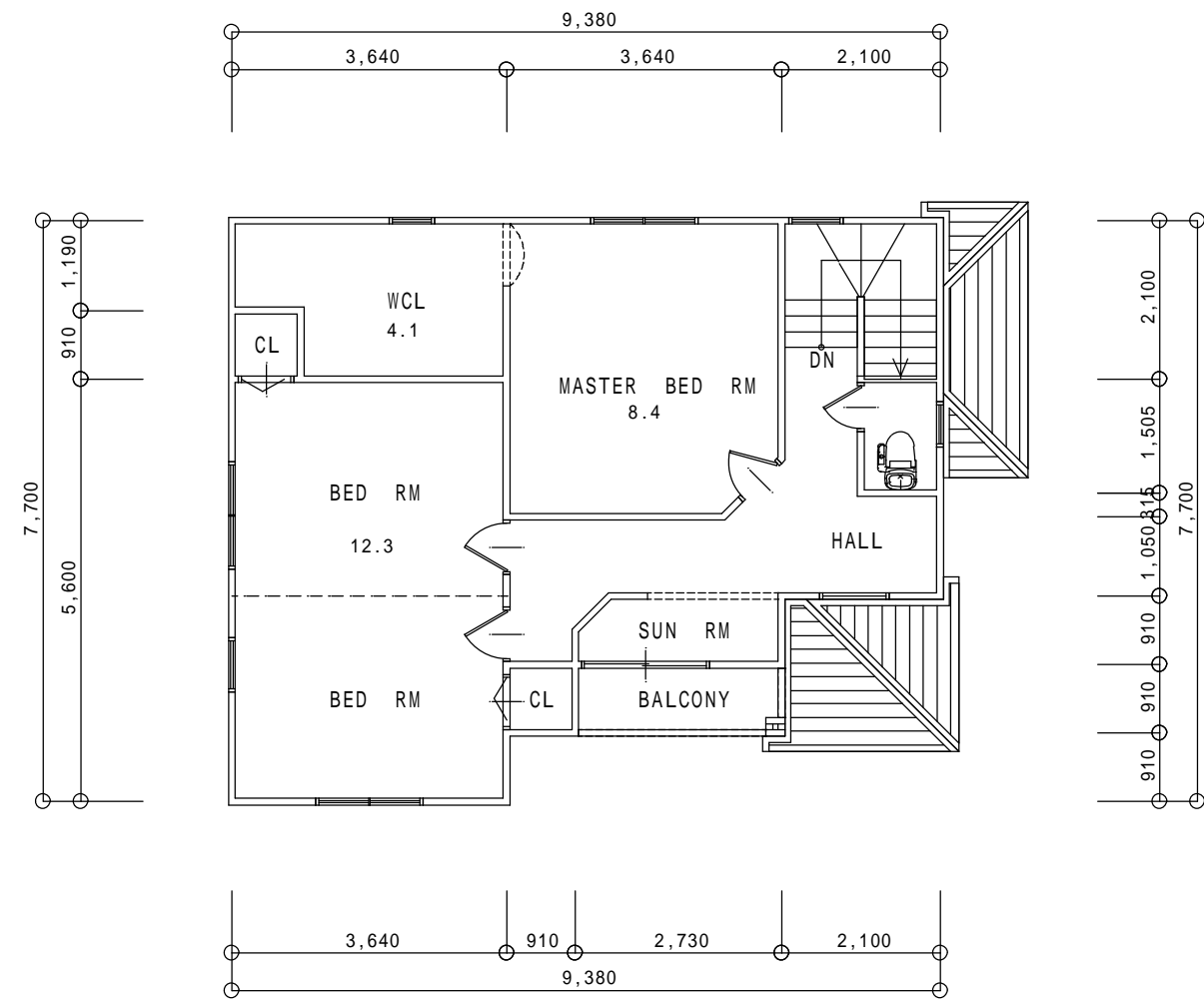
2nd FLOOR PLAN S:1/100
