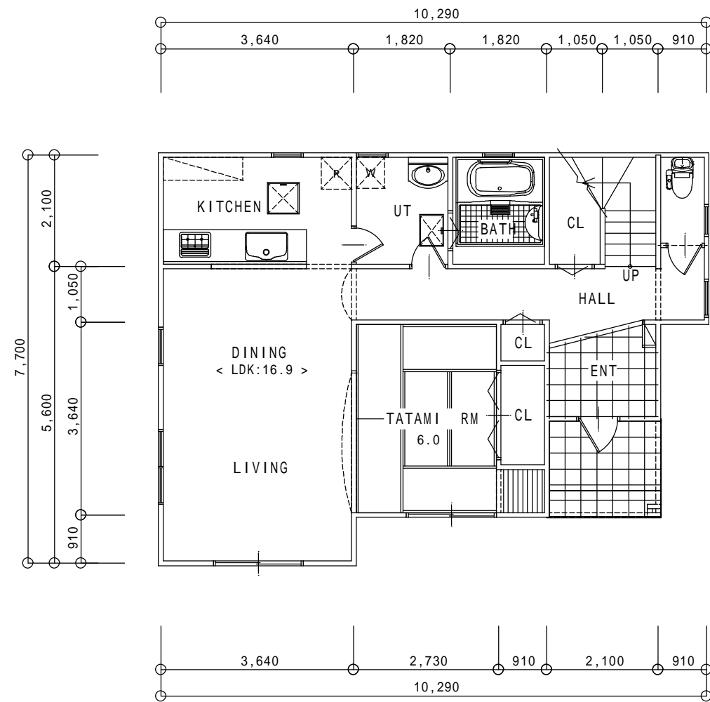
1st FLOOR PLAN S:1/100
