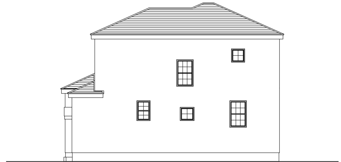
WEST ELEVATION S : 1 / 100
