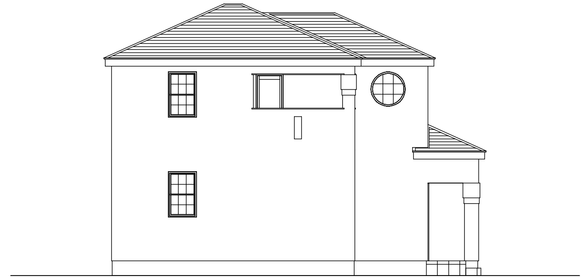
EAST ELEVATION S : 1 / 100
