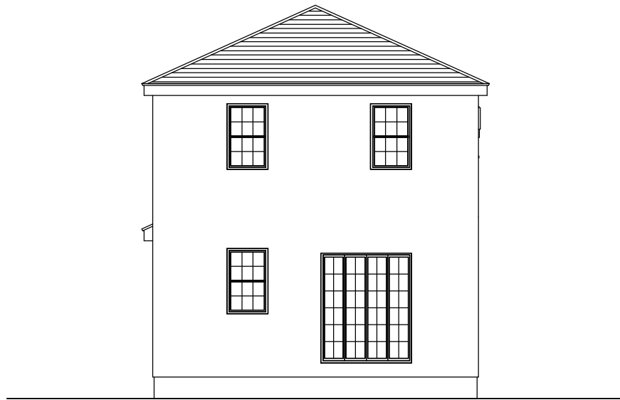
SOUTH ELEVATION S : 1/ 100
