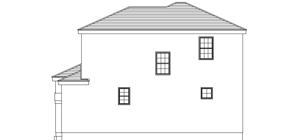
WEST ELEVATION S : 1/ 100
