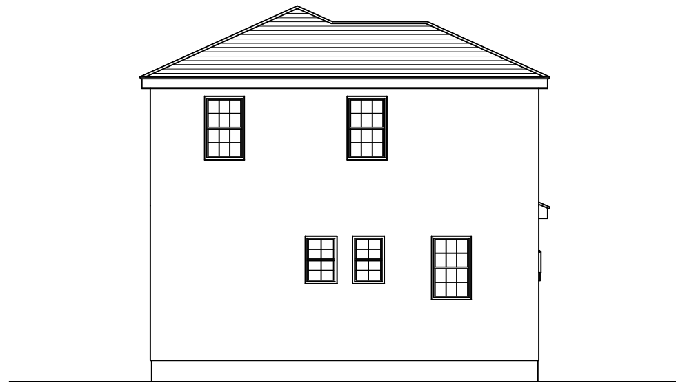
NORTH ELEVATION S: 1/100
