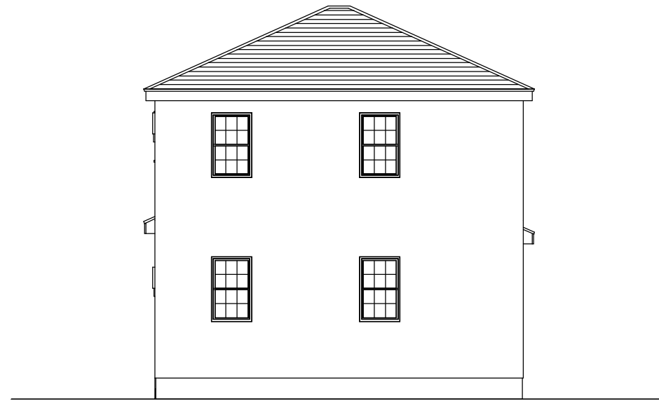
EAST ELEVATION S : 1/ 100
