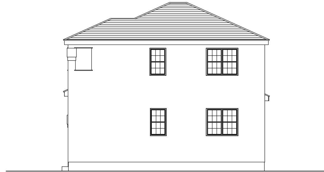
EAST ELEVATION S : 1 / 100
